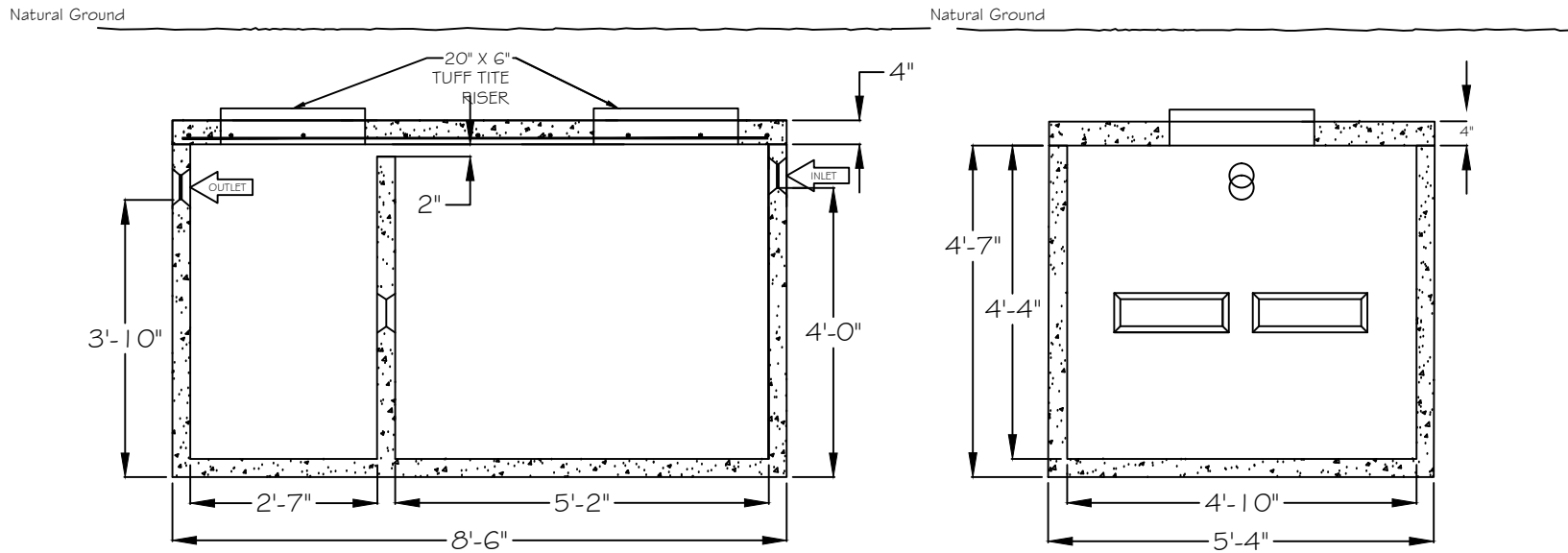
ELEVATION VIEW
