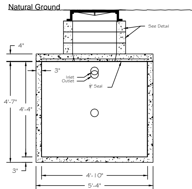
END VIEW
