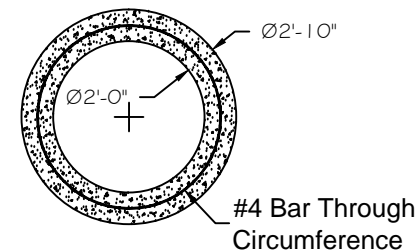
GRADE RING - PLAN VIEW
