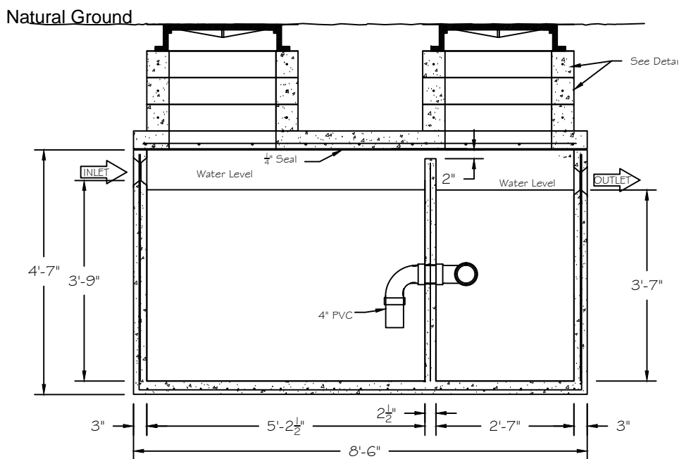
ELEVATION VIEW
