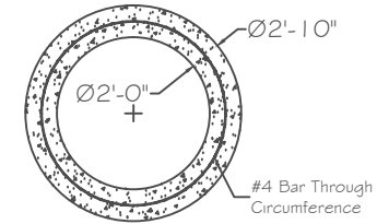
GRADE RING -PLAN VIEW
