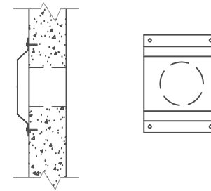
VENT DETAIL
